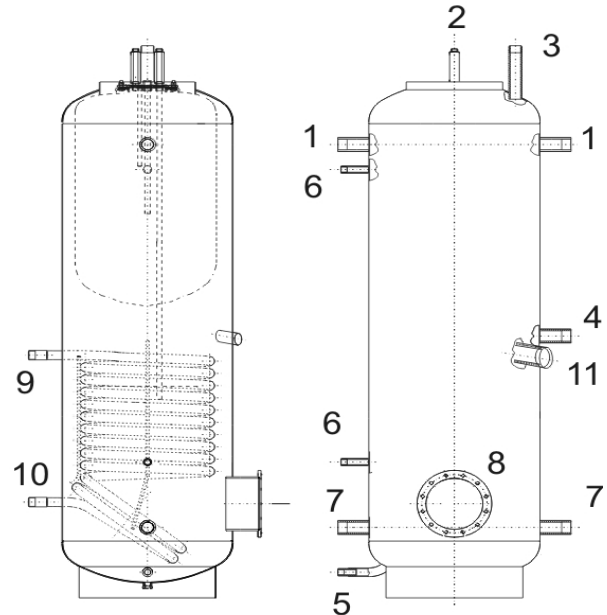
NADO v2 - with inner vessel 140 l
